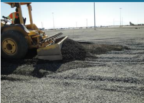
Installing crushed aggregate in the GEOWEB sections with 2 in surface course
